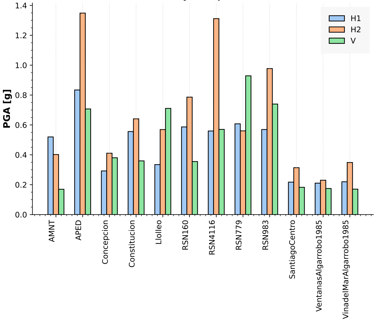
PGA by Component
